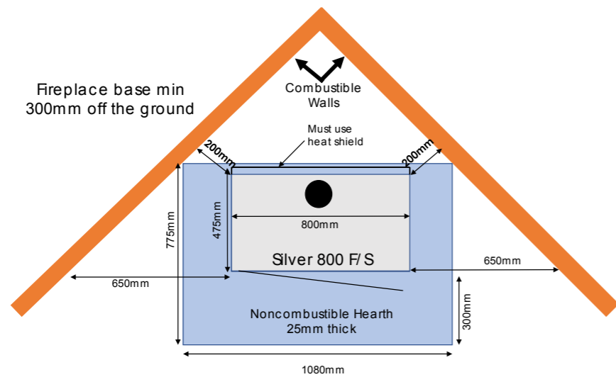
Silver 800 F/S Clearance Diagram Corner
