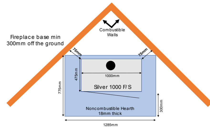
Silver 1000 F/S Clearance Diagram Corner
