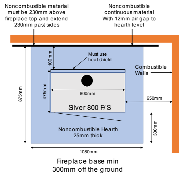
Silver 800 F/S Clearance Diagram Corner
