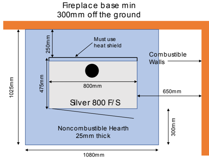
Silver 800 F/S Clearance Diagram
