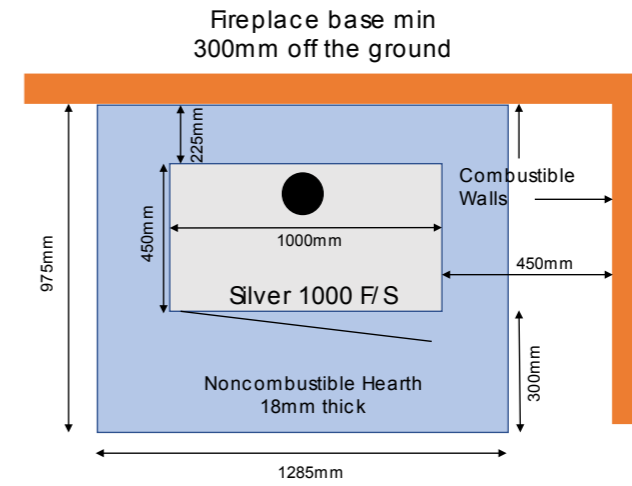
Silver 1000 F/S Clearance Diagram
